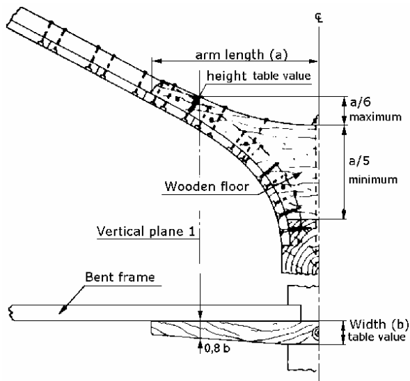
Figure 3 (Timber floor)
