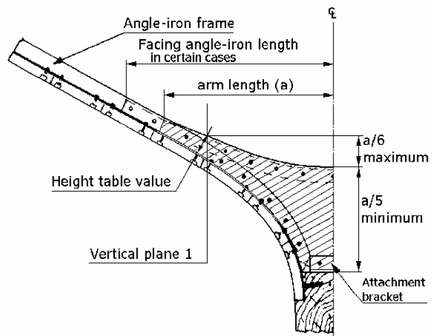
Figure 4 (Angle-iron floor)
